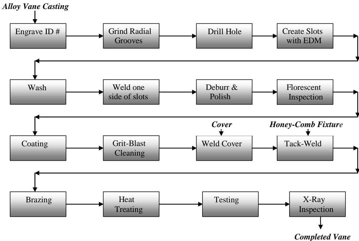
Figure 2: Valve Production Process Map
