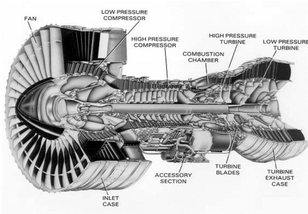
Figure 1: PW4000 Turbojet Engine
