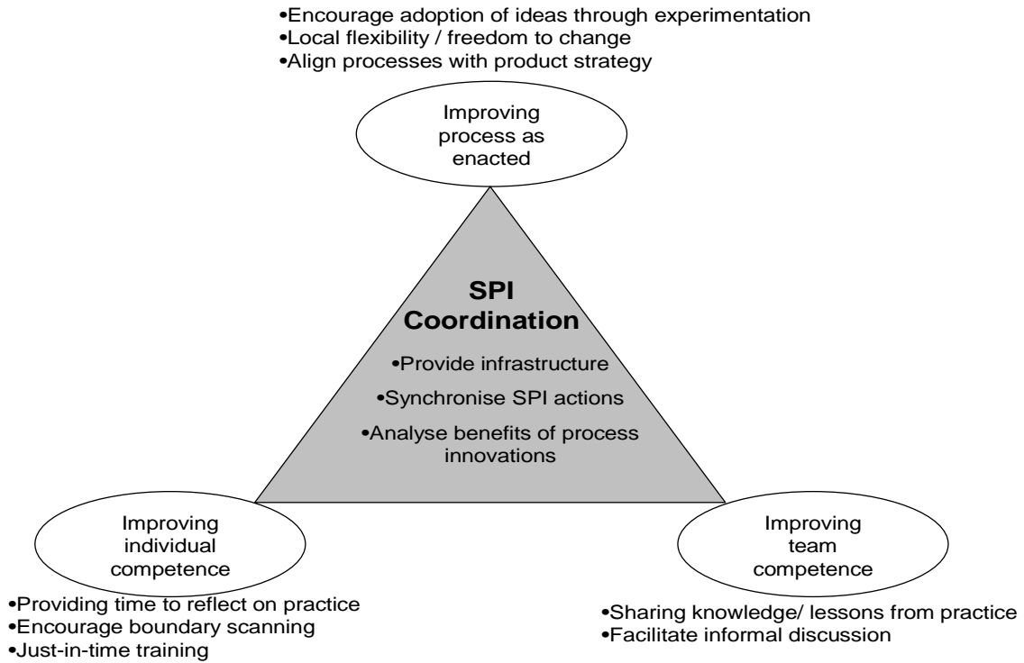
Figure 1: A model of an agile SPI method.
